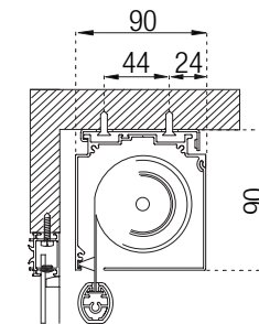
Attacco a soffitto con supporti Ceiling mounting with brackets
