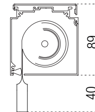
Fondale intascato Pocketed bottom rail
