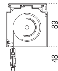
Fondale 11x41 11x41 bottom rail
