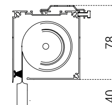
Fondale intascato Pocketed bottom rail
