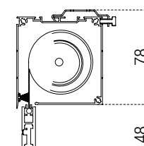
Fondale 11x41 11x41 bottom rail
