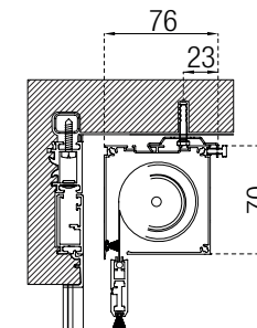
Attacco a soffitto con supporti Ceiling mounting with brackets
